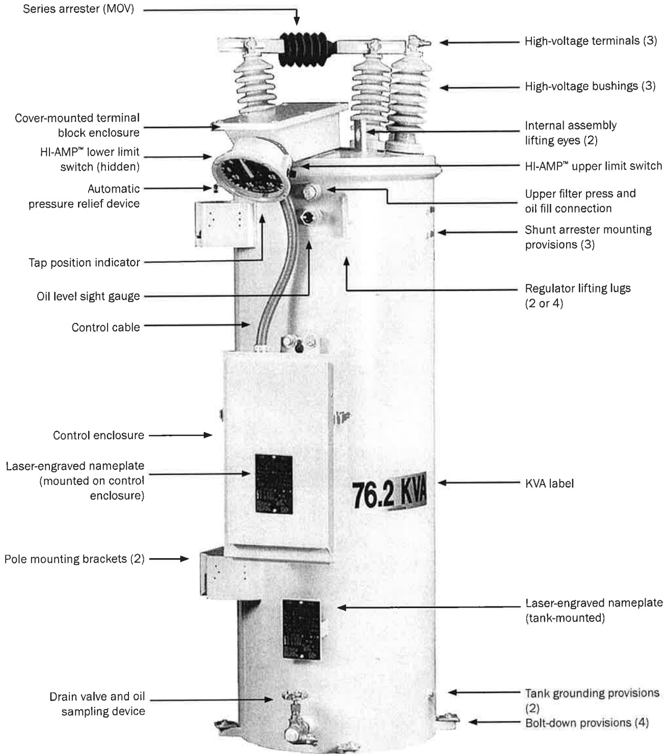
FIGURE 4: SVR-1 single-phase step voltage regulator standard features and accessories (overhead type as shown)
